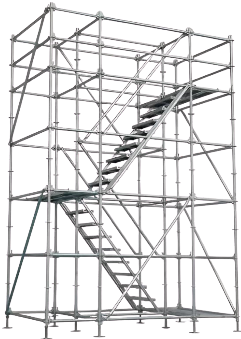
Ringlock System
